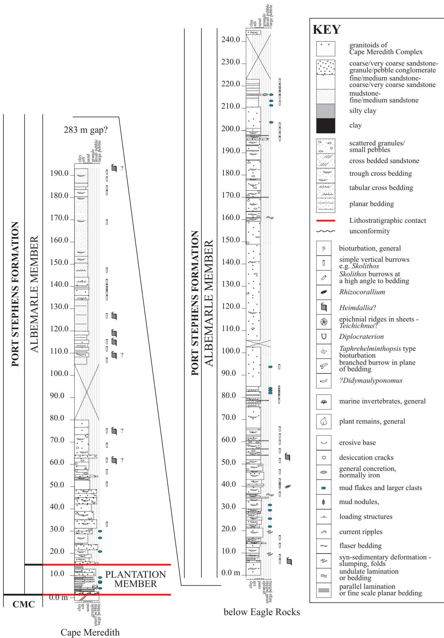
Appendix 1. Logs of the Port Stephens Formation, section locality indicated below each section (Fig. 5). Long diagonal lines join sections.
