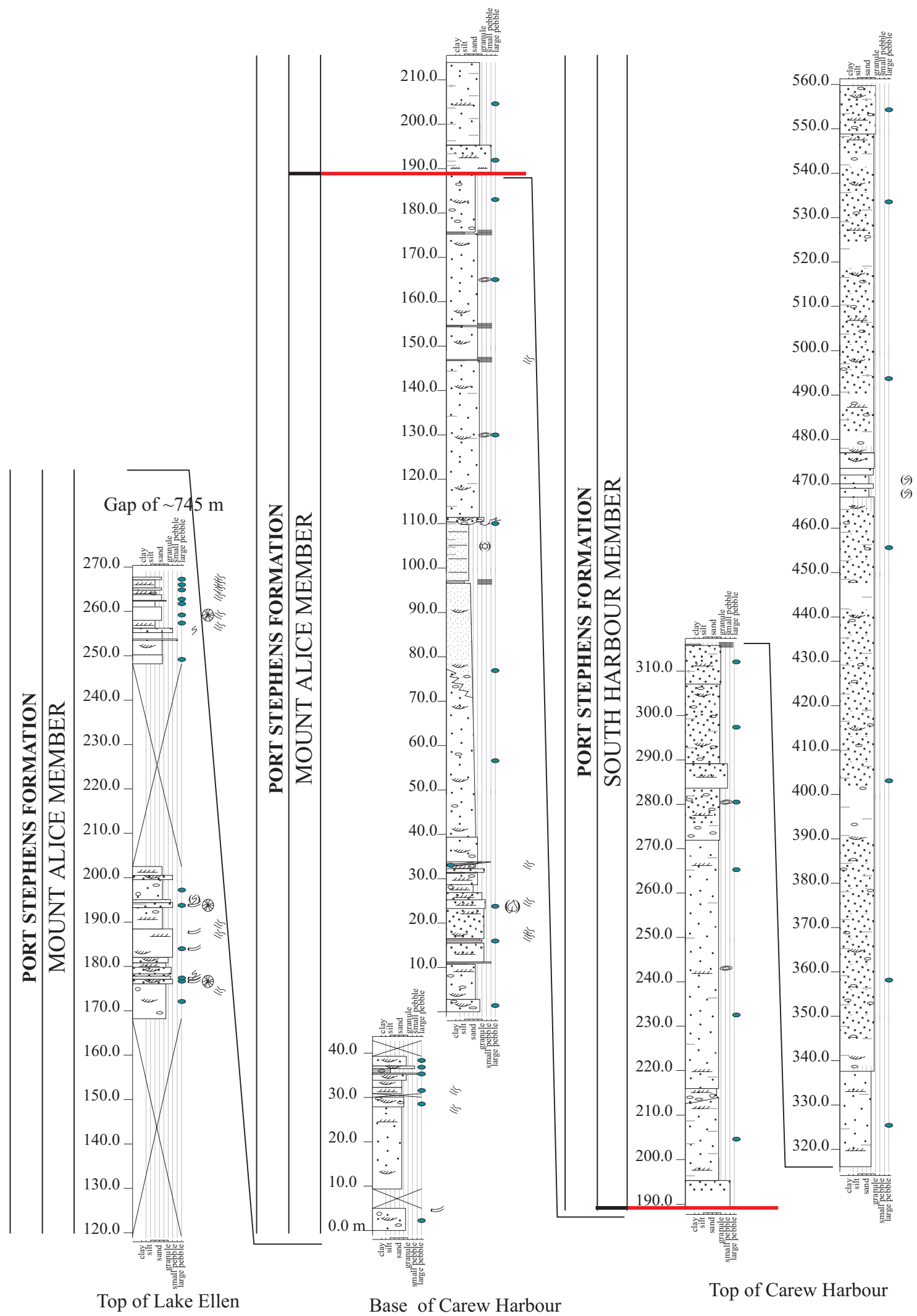
1c. Top of the Mount Alice Member, showing the gradational change to the South Harbour Member.
