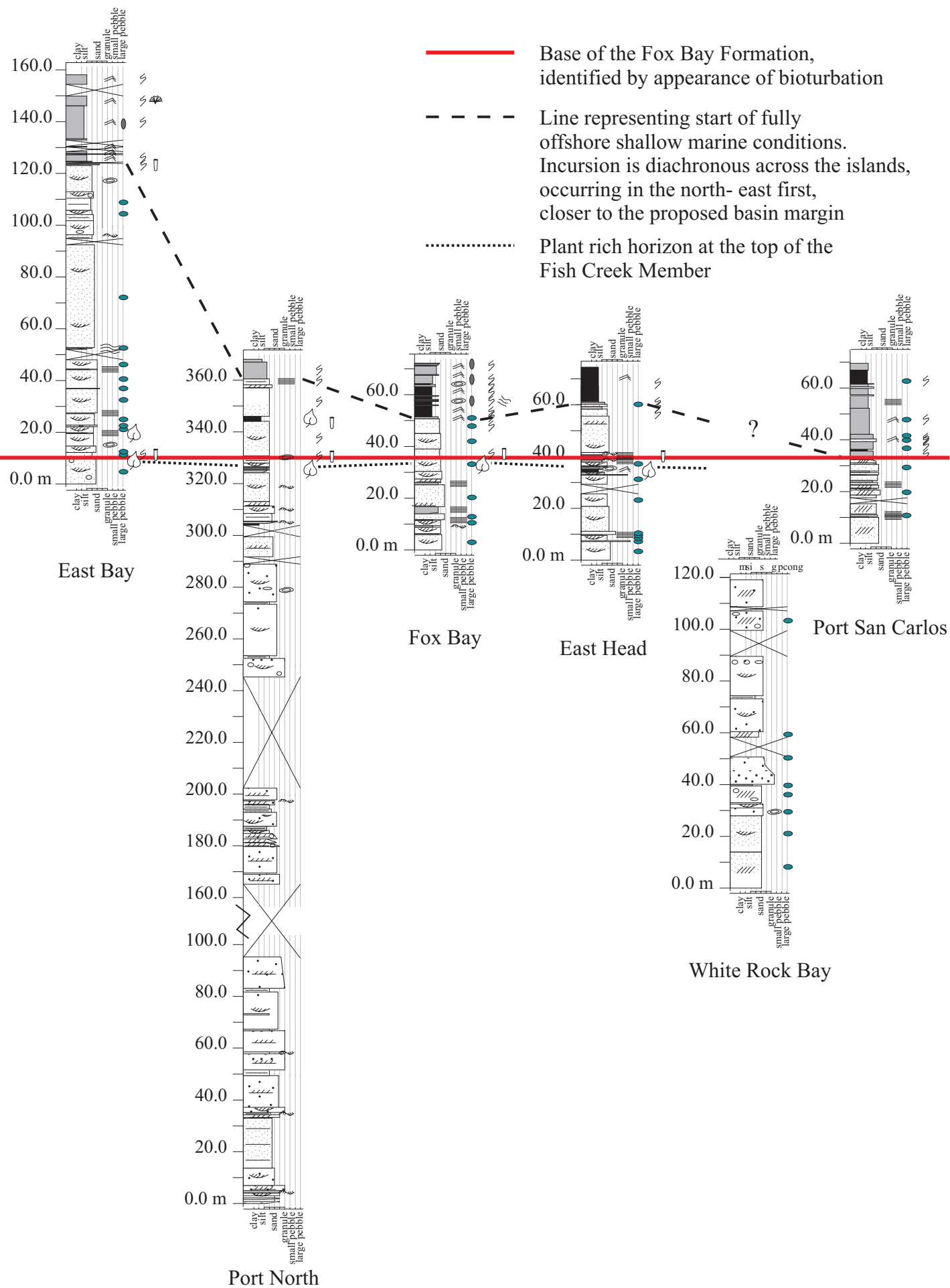
Appendix 2. Logs of the Fish Creek Member, locality indicated with each section. Sections ordered approximately from south-west to north-east across West and East Falkland. For key see Appendix 1.
