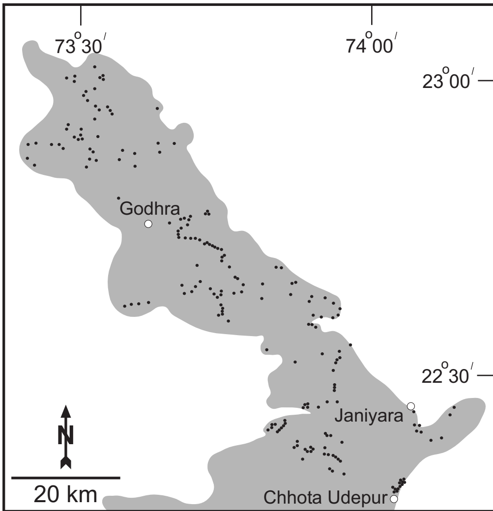
Supplementary data-1: Map showing locations of sites from where granite samples were taken. A total of 202 sites in the granite were sampled. On the present scale, closely located sites have not been shown.
