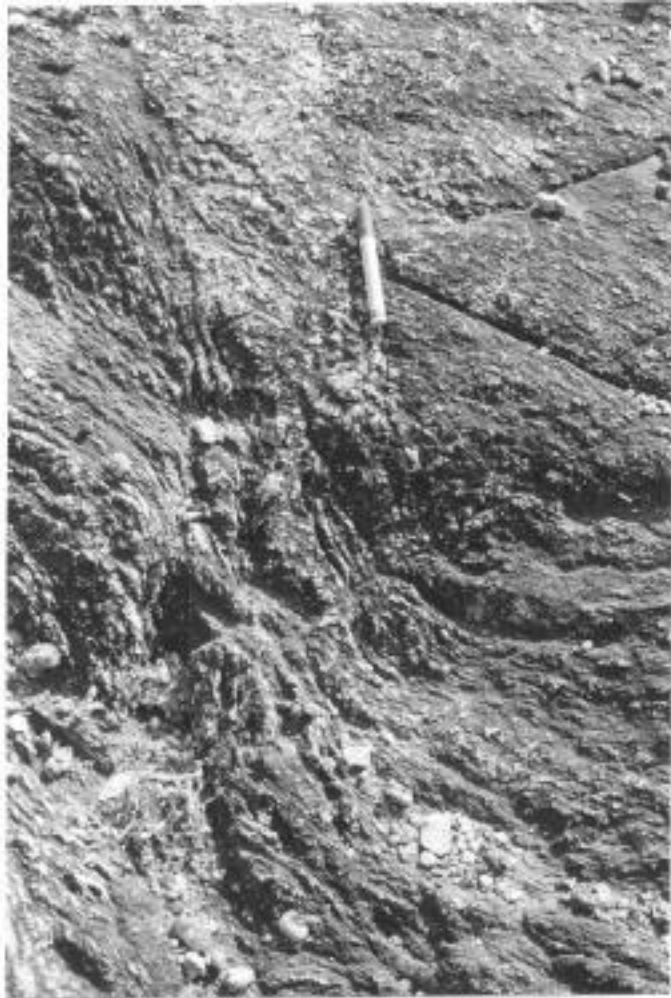
Supplementary data-2: Field photograph of high-strain zone at the contact between granite and gneiss. Camera faces ESE
