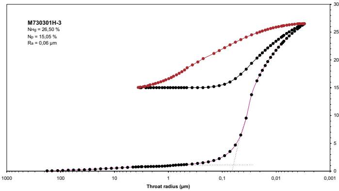
Mercury Porosimetry M730301H-3
