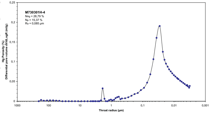
Mercury Porosimetry M730301H-4
