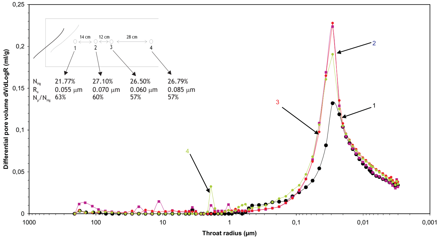
Mercury Porosimetry M730301H-1
