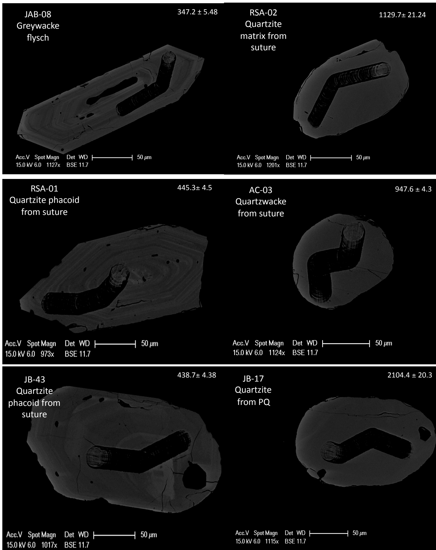
Supplementary Figure 1. Selected SEM backscatter images of representative detrital grains from the PDLZ and SPZ
